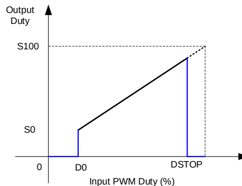
Figure 3: Stop at High Duty Cycle
