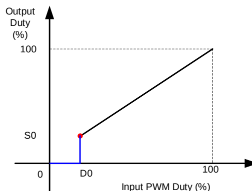
Figure 2: Minimum Speed
