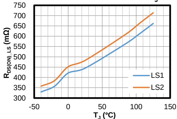
LS-FET On Resistance vs. T_J
