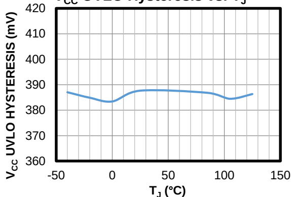
V_{CC} UVLO Hysteresis vs. T_J
