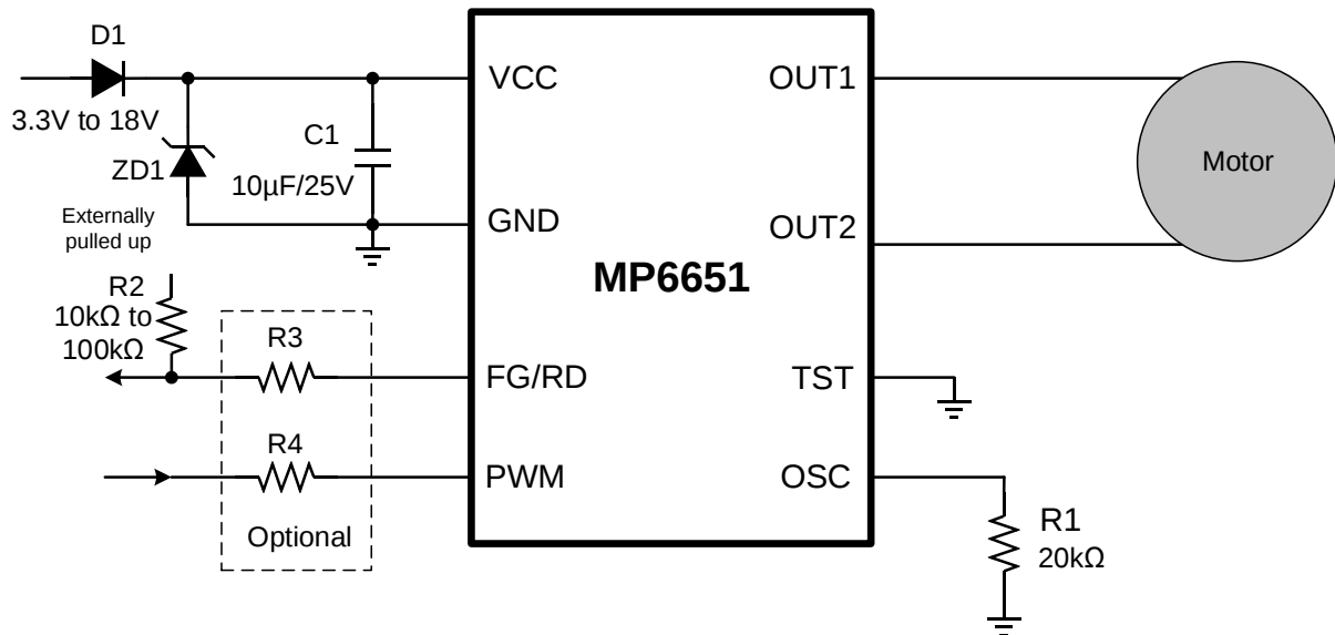
Figure 11: Typical Application Circuit
