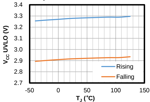
V_{CC} UVLO vs. Junction Temperature
