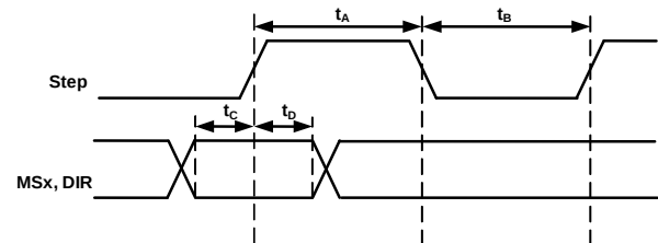
Figure 3: STEP Input Timing
