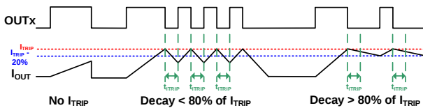
Figure 2: Current Regulation
