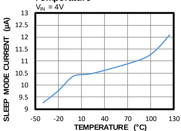
Sleep Mode Current vs. Temperature V_{IN} = 4V
