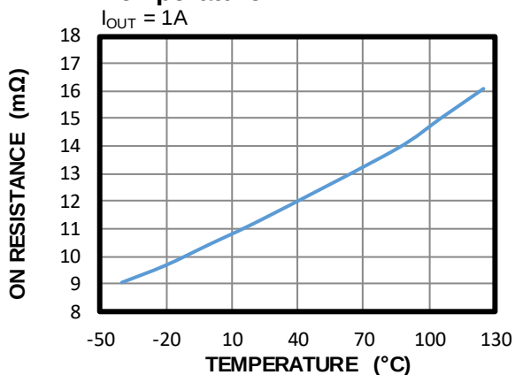
LS-FET On Resistance vs. Temperature I_{OUT} = 1A
