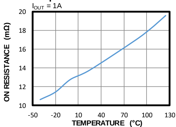
HS-FET On Resistance vs. Temperature I_{OUT} = 1A
