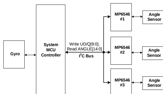
Figure 7: Multi-Slave Bus Connection
