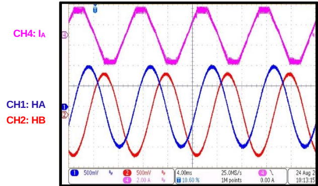
Steady State PWM duty at 100%
