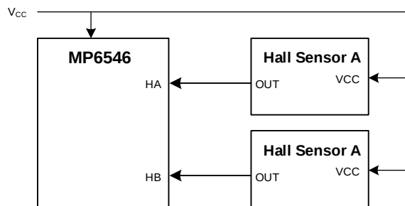
Figure 5: Linear Hall Sensor Interface
