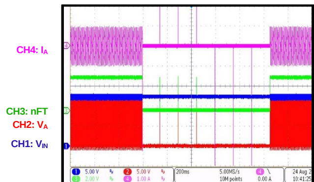
Short-Circuit Protection Short UA and UB
