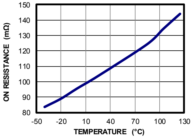
LS On Resistance vs. Temperature I_{OUT} = 1A
