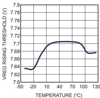
VREG Rising Threshold vs. Temperature
