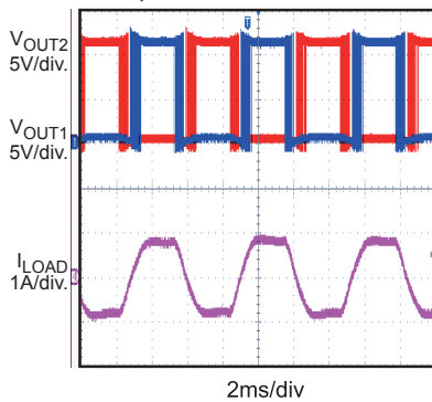
Typical Waveform, Shutdown with PWM
