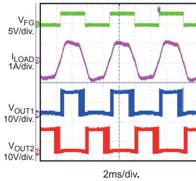
Typical Waveform, Enable Soft On & Soft Off
