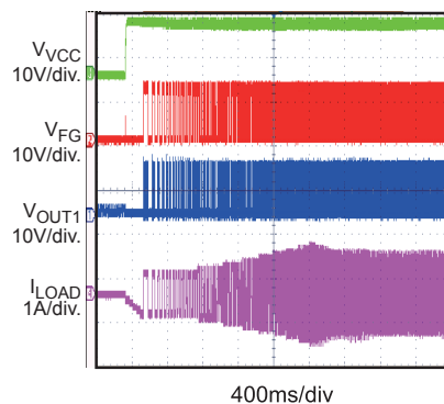
Typical Waveform, Start Up with V CC
