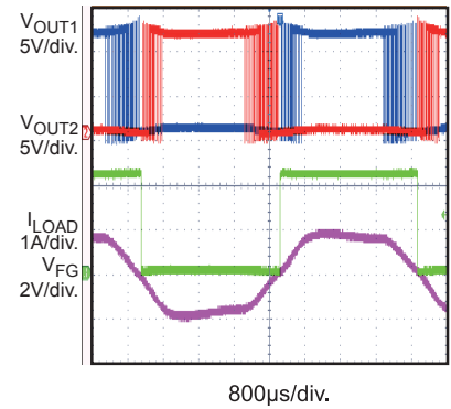
Typical Waveform, Start Up with PWM
