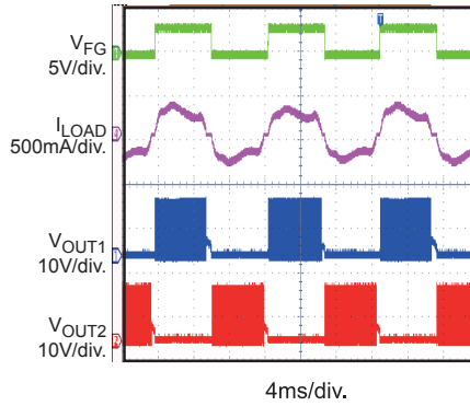
Typical Waveform, Disable Soft On & Soft Off
