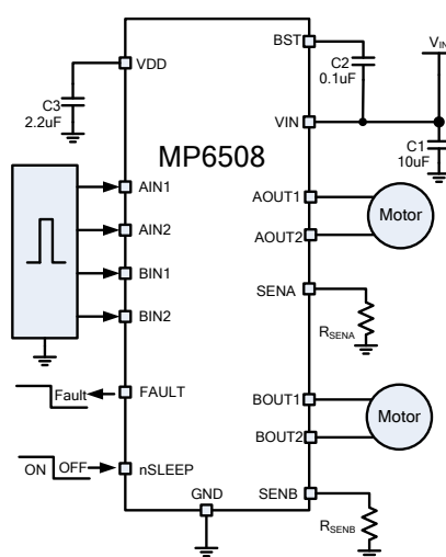
Dual DC Motor Application
