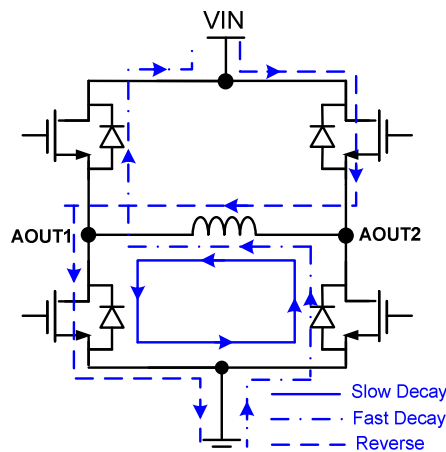
Figure 3: Reverse Operation
