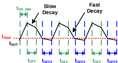
Figure 5: Current Regulation of Low Current/Low Inductance
