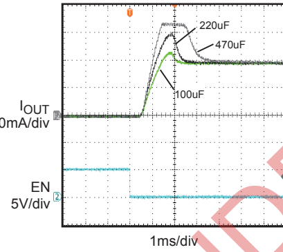
Inrush Current with Different Load Capacitance I_{OUT}=1A
