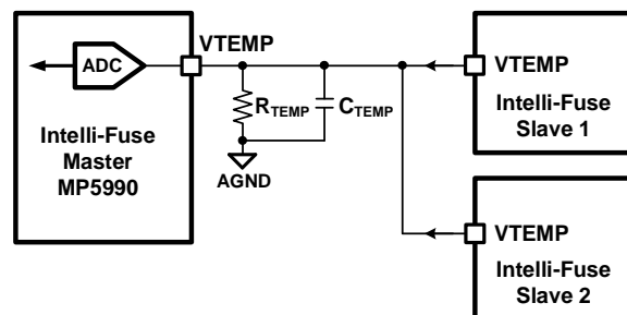
Figure 13: Multi-Fuse Temperature-Sense in Parallel Operation
