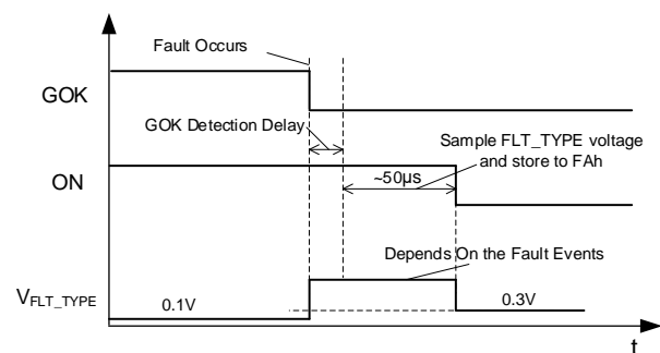
Figure 14: FLT_TYPE Indication
