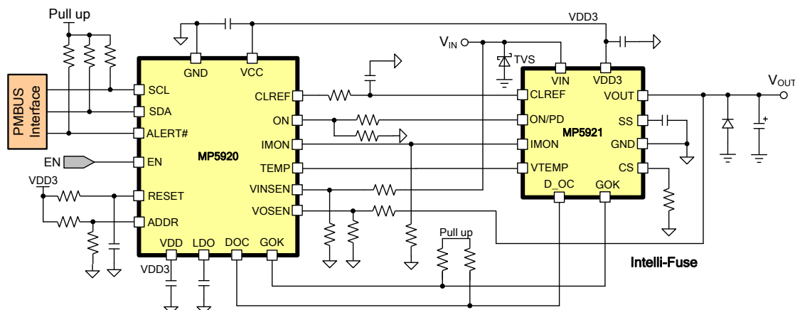
MP5921 Controlled by Hot-Swap Controller
