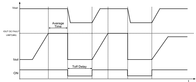
Figure 6: OCP Fault Operation
