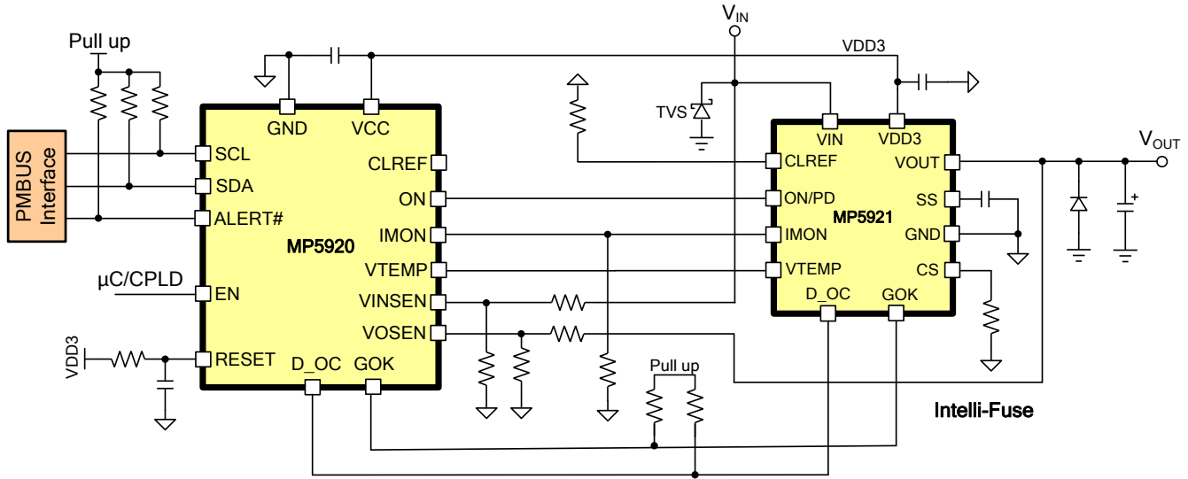
MP5920 + MP5921 with Static Max Current Limit
