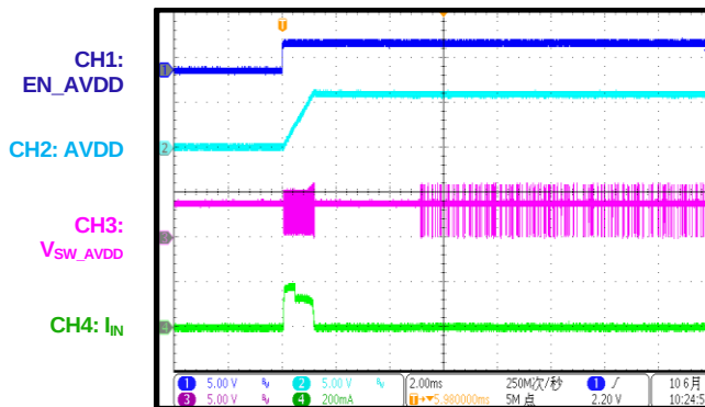
AVDD Start-Up
