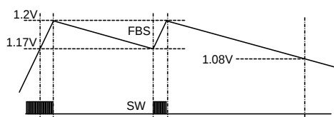
Figure 4: Boost Charge Mode
