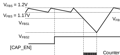
Figure 7: Capacitor Health Test
