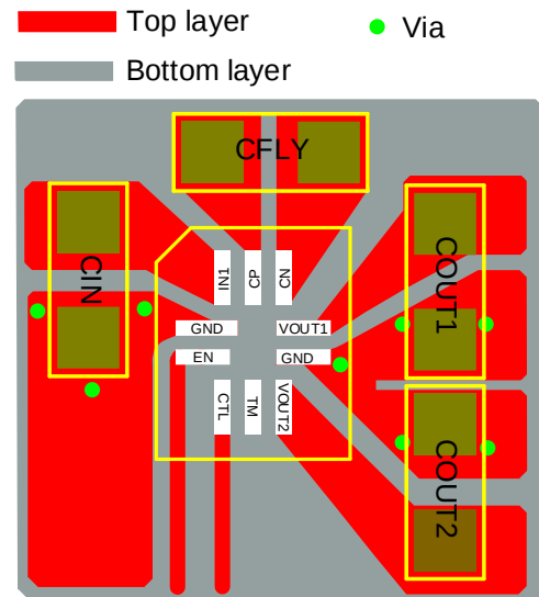
Figure 3: Recommended PCB Layout
