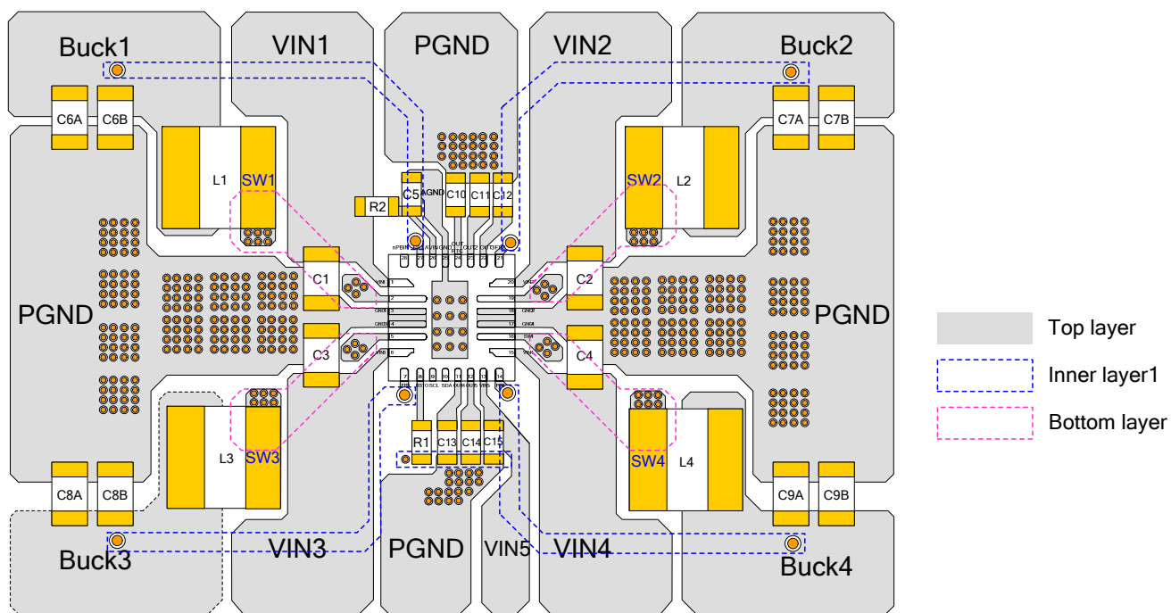
Figure 14: Recommended Layout (14)
