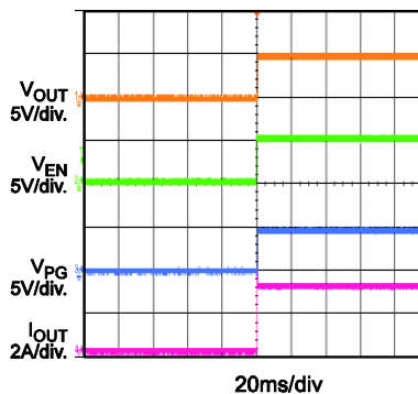
EN Start-Up (Load Switch)
