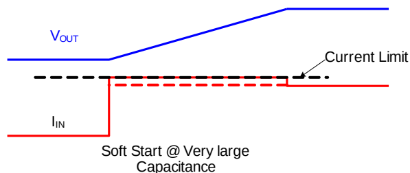
Figure 3: Soft Start Periods at different output capacitance
