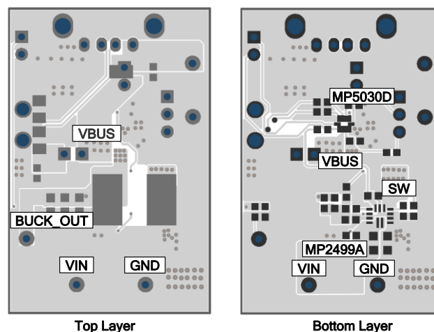
Figure 6: Recommended Layout
