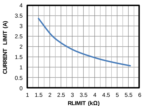
Current Limit vs. R_{LIMIT}
