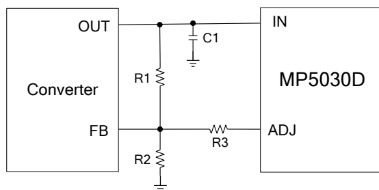
Figure 5: V_{ADJ} -Set Maximum V_{OUT}
