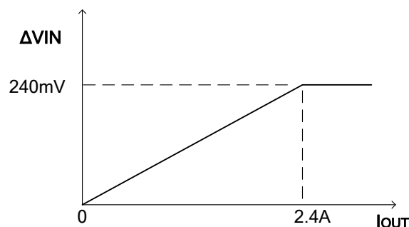
Figure 2: Line Drop Compensation
