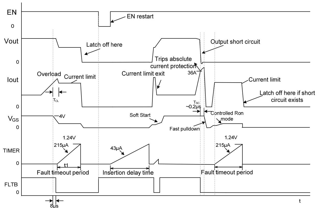
Figure 2: Over-Current Protection
