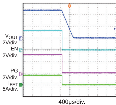
Shutdown through EN I_{OUT}=3.8A , with PD
