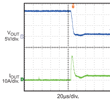
0.3 \Omega Load Connected To Enabled Device
