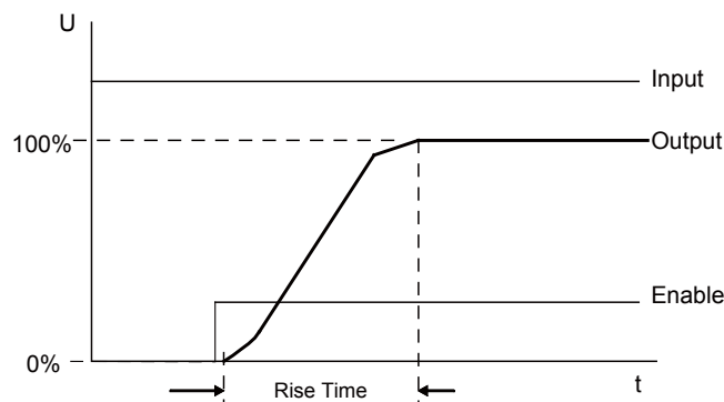
Figure 2—Rise Time
