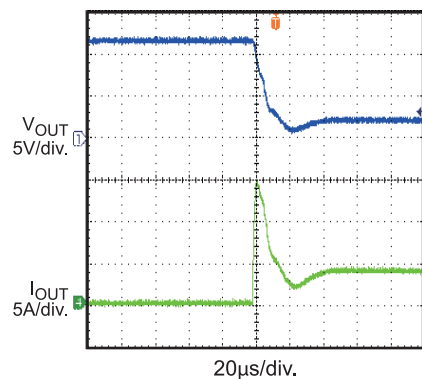
0.6 \Omega Load Connected To Enabled Device
