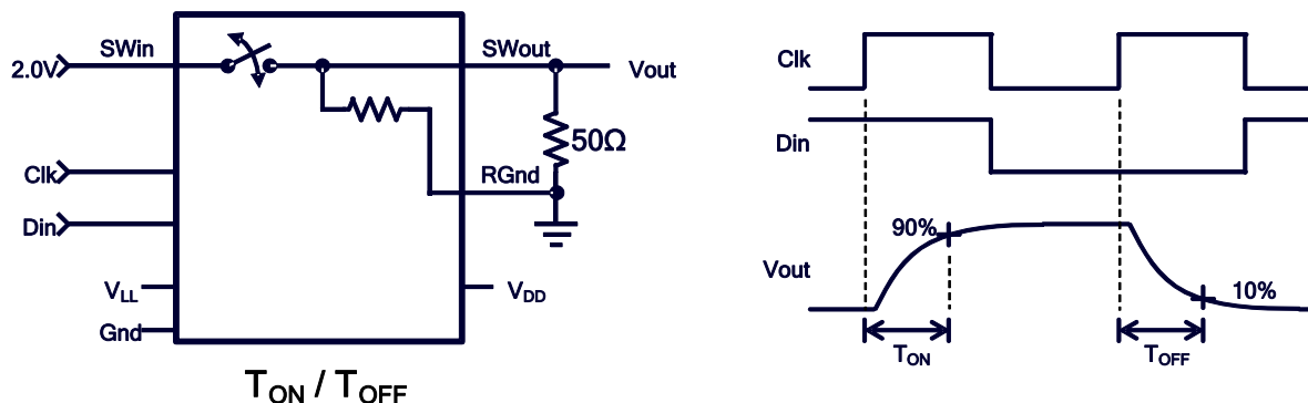
Test Circuit 5
