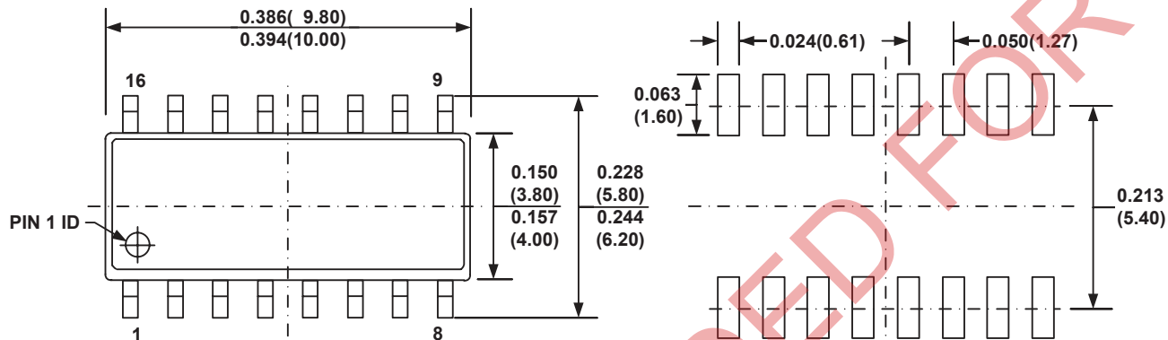
TOP VIEW
