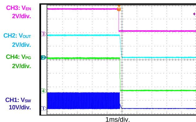
PG Shutdown through EN I_{OUT} = 6A
