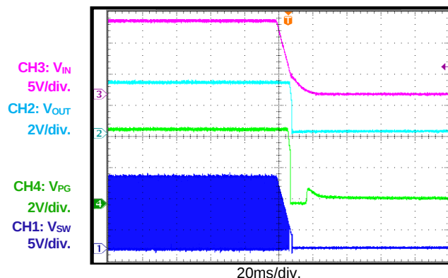
PG Shutdown through VIN I_{OUT} = 6A
