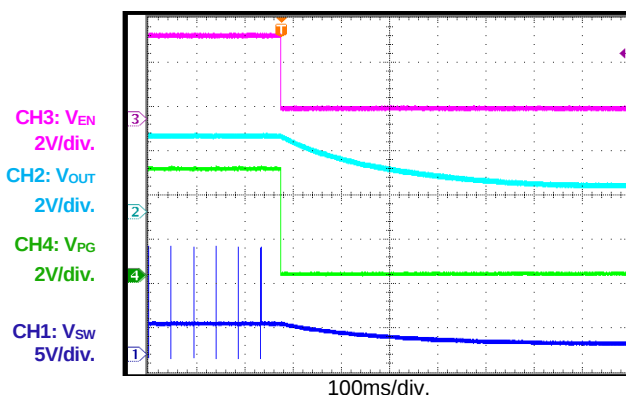
PG Shutdown through EN I_{OUT} = 0A
