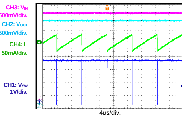
Low-Dropout Mode
