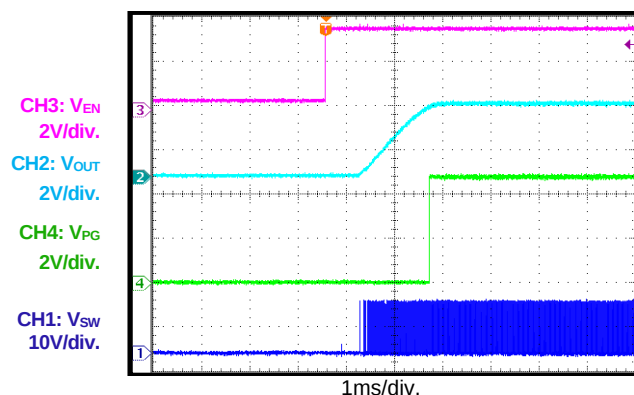
PG Start-Up through EN I_{OUT} = 6A
