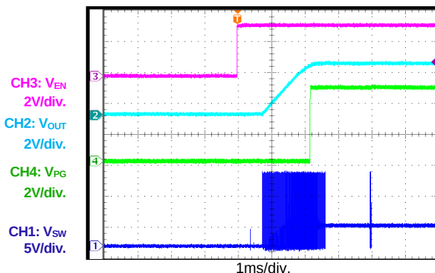
PG Start-Up through EN I_{OUT} = 0A
