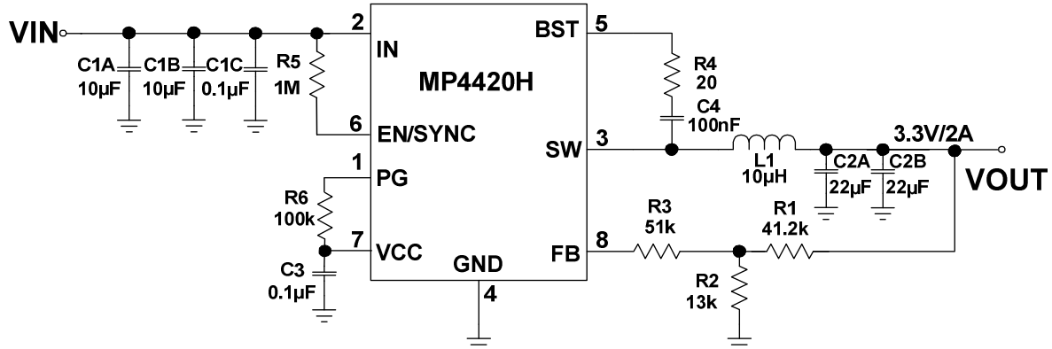
Figure 8: 3.3V Output Typical Application Circuit
