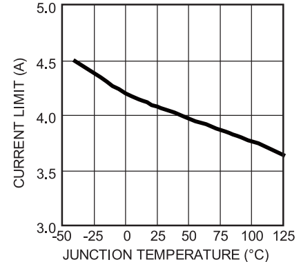
Current Limit vs. Junction Temperature V_{IN}=12V , Duty Cycle=40%
