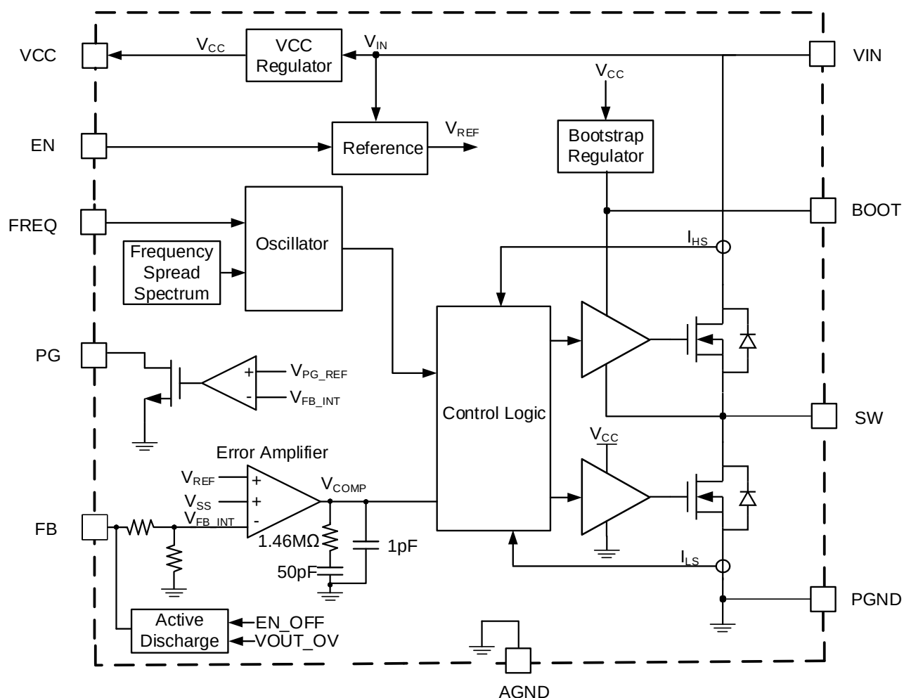
Figure 4: Functional Block Diagram (Fixed Output)
