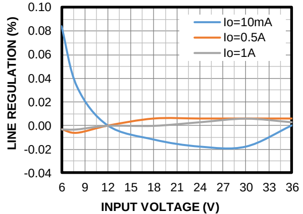
Line Regulation
