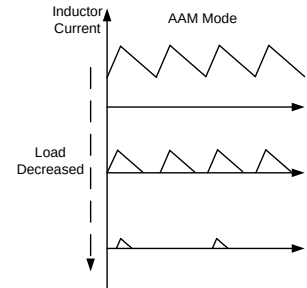
Figure 5: AAM Mode
