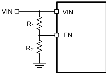
Figure 9: Configurable UVLO via the EN Divider
