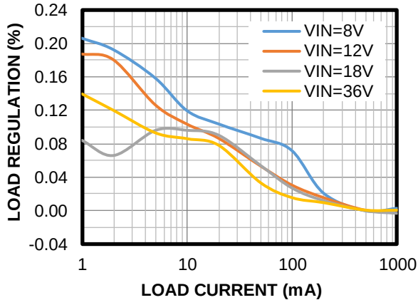
Load Regulation
