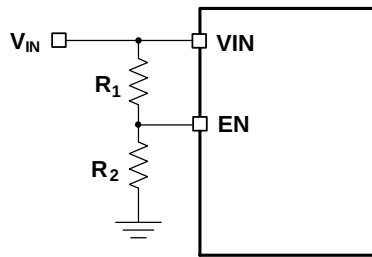
Figure 10: Configurable UVLO via the EN Divider
