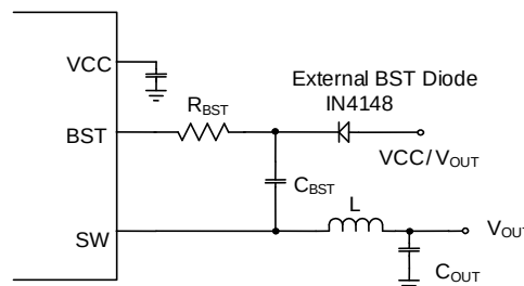
Figure 8: Optional External Bootstrap Diode to Enhance Efficiency
