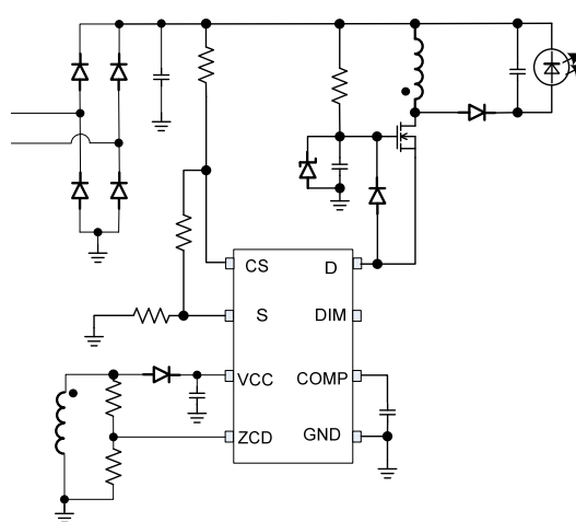
Non-Isolated Buck-Boost Application
