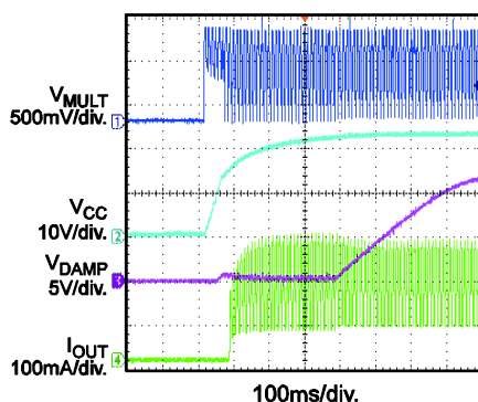
V IN Start Up V IN =230V AC /50Hz, Full Load
