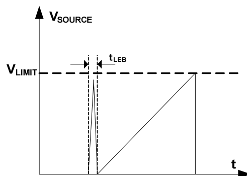
Figure 5: Leading Edge Blanking (LEB)
