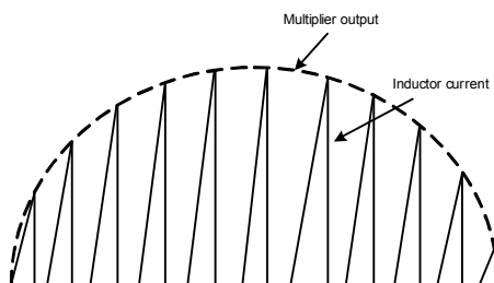
Figure 4: Power-Factor Correction
