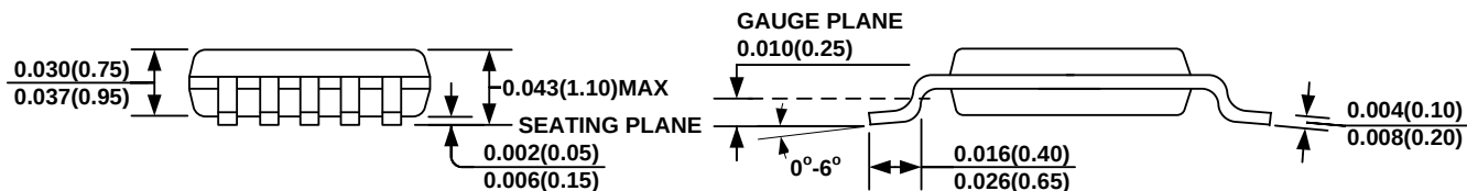
FRONT VIEW
