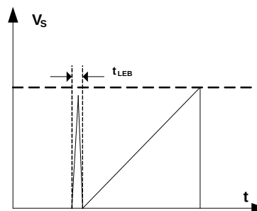
Figure 6: Leading-Edge Blanking
