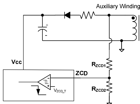
Figure 3: Zero-Current Detector
