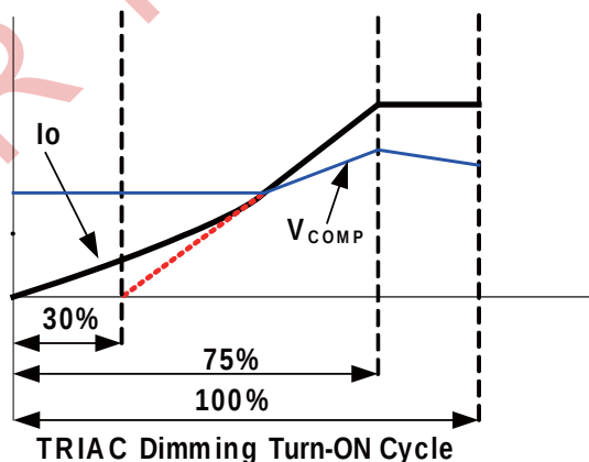
Figure 13: Dimming Curve
