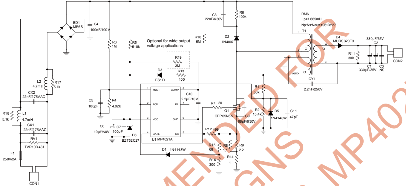
Figure 15—Universal Input, Isolated Flyback Converter, Drive 3-6 LEDs in Series, 350mA LED Current for LED Bulb Lighting
