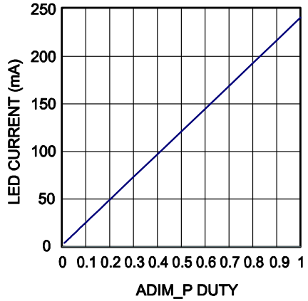
Pulse-Input Analog Dimming
