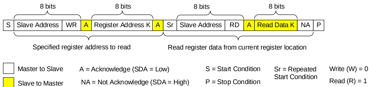
Figure 6: I 2 C Read Single Register Example
