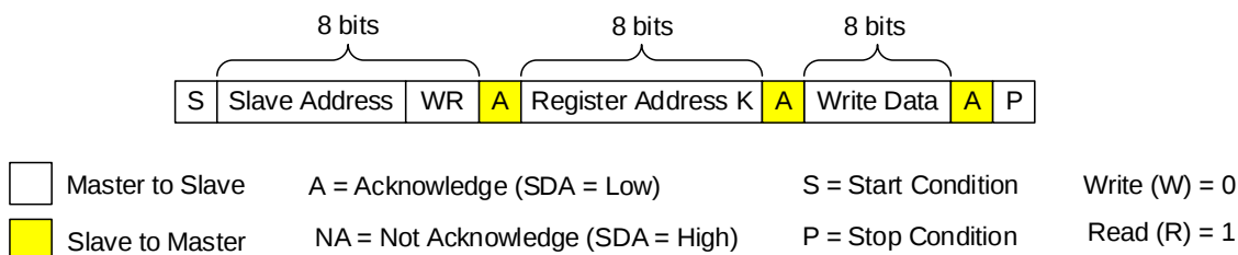
Figure 5: I 2 C Write Single Register Example
