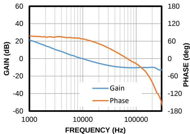
Bode Plot
