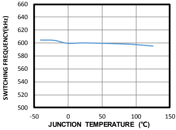
Switching Frequency vs. Junction Temperature
