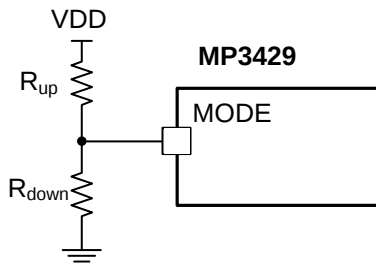
Figure 3: MODE Setting
