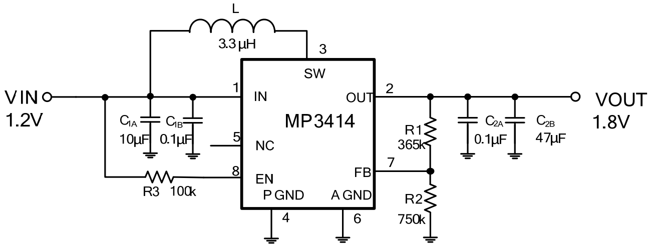
Figure 3: Boost Circuit. V_{IN}=1.2\text{V} , V_{OUT}=1.8\text{V} .
