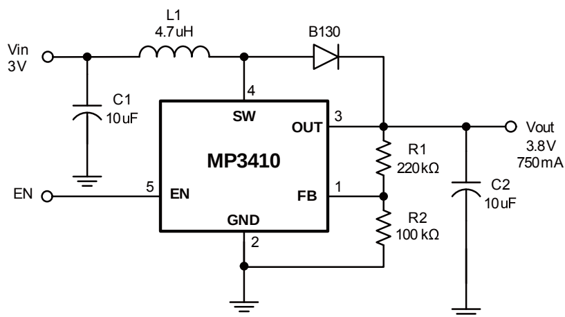
Figure 6—3V-3.8V/750mA Application
