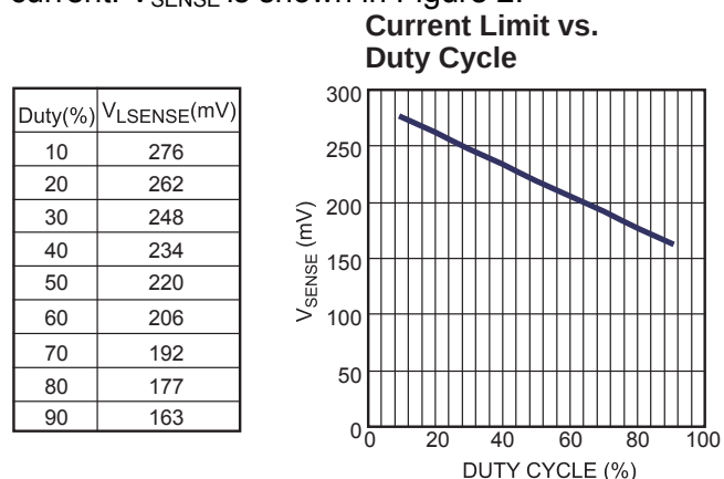
Figure 2: V_{SENSE} vs Duty Cycle
