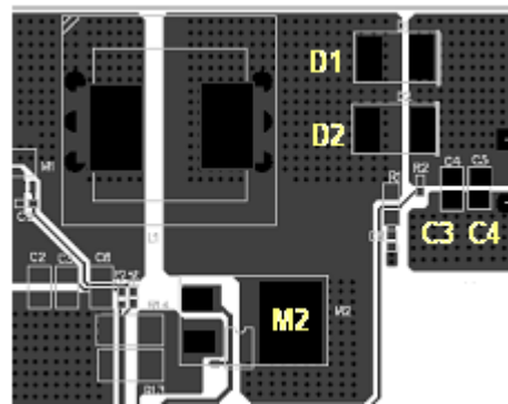
Figure 3: Layout Suggestion
