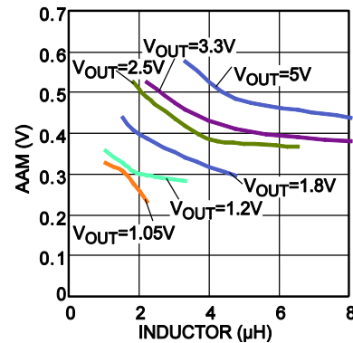
Figure 7—AAM selection for common output voltages ( V_{IN2} = 4.5 \text{ V} - 24 \text{ V} )
