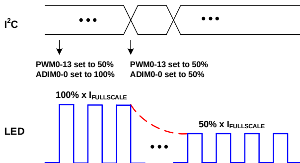
Figure 12: PWM Dimming from I 2 C Interface
