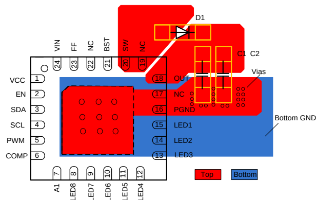
Figure 21: Recommended PCB Layout
