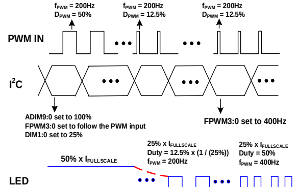
Figure 13: Mixed Dimming from PWM Input
