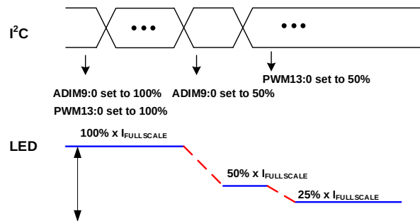
Figure 10: Analog Dimming from I²C Interface
