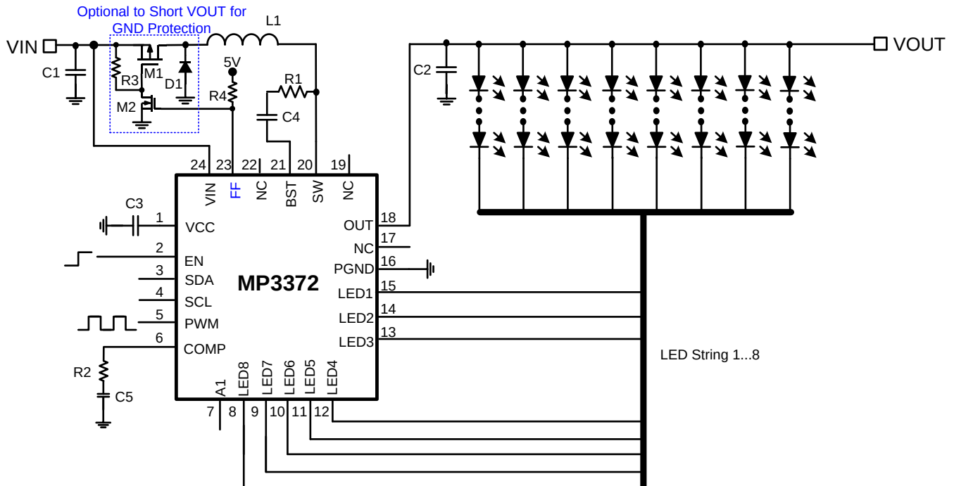
Figure 2: Add External MOSFET to Disconnect VOUT from VIN when VOUT is Shorted to GND
