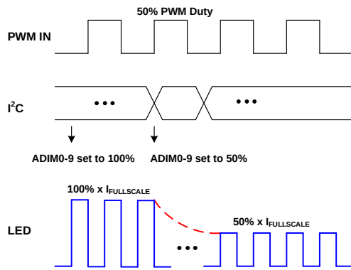
Figure 11: PWM Dimming from PWM Input
