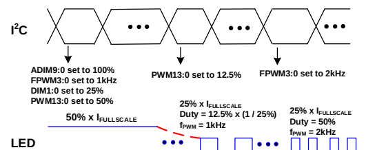
Figure 14: Mixed Dimming from the I 2 C Interface Phase Shift PWM Dimming
