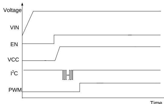
Figure 5: Recommended Start-Up Sequence
