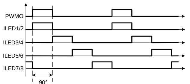
Figure 17: Phase Shift with 4 Channels
