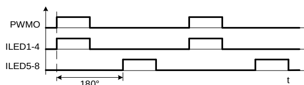
Figure 19: Phase Shift with 2 Channels
